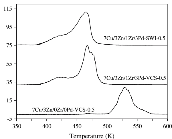
Fig. 7 Hydrogen TPR profiles for catalysts 7\text{Cu}/3\text{Zn}/0\text{Zr}/0\text{Pd-VCS-0.5} (bottom), 7\text{Cu}/3\text{Zn}/1\text{Zr}/3\text{Pd-VCS-0.5} (middle), and 7\text{Cu}/3\text{Zn}/1\text{Zr}/3\text{Pd-SWI-0.5} (top)
