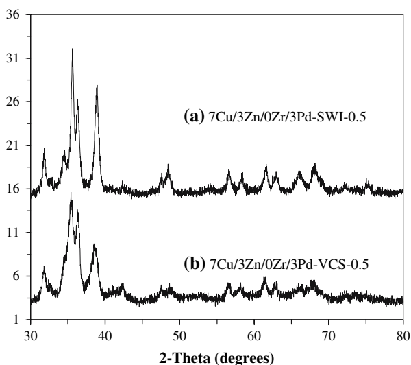
Fig. 6 XRD patterns of catalysts with composition prepared by SWI and VCS methods (a) 7\text{Cu}/3\text{Zn}/0\text{Zr}/3\text{Pd-SWI-0.5} , (b) 7\text{Cu}/3\text{Zn}/0\text{Zr}/3\text{Pd-VCS-0.5}
